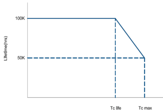
Lifetime vs. Temperature Curve
