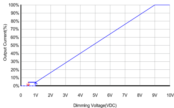
Dimming curve
